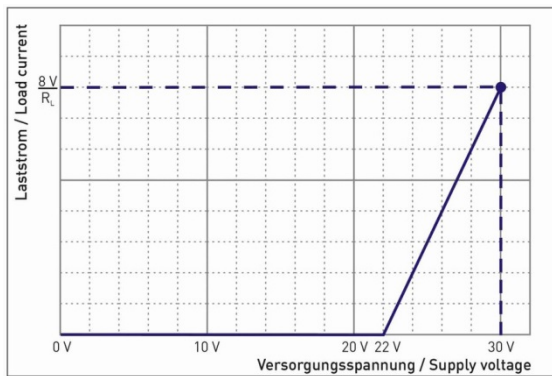
Load current
