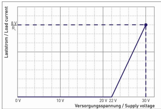
Laststrom
